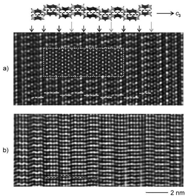
Figure 4. HRTEM studies on 3 (a), zone axis [100]_{\text{trig}} with inserted micrograph ( \text{occ.}(\text{Bi})_{18h} = 1 , \text{occ.}(\text{Sn})_{18h} = 0 , \text{occ.}(\text{Bi})_{9e} = 0 , \text{occ.}(\text{Sn})_{9e} = 1 , \Delta f = -65 \text{ nm} , t = 7.3 \text{ nm} ). b) Structure variant with a repeating unit of 50 Å.
